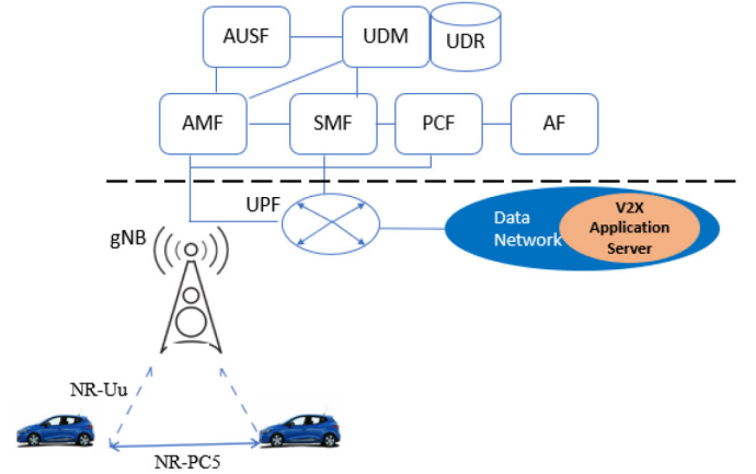
Fig. 3. 5G system architecture for V2X communications.
